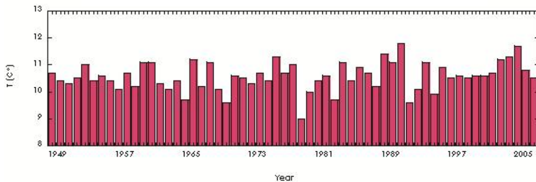
July main temperature - Fagurhólmsmýri
